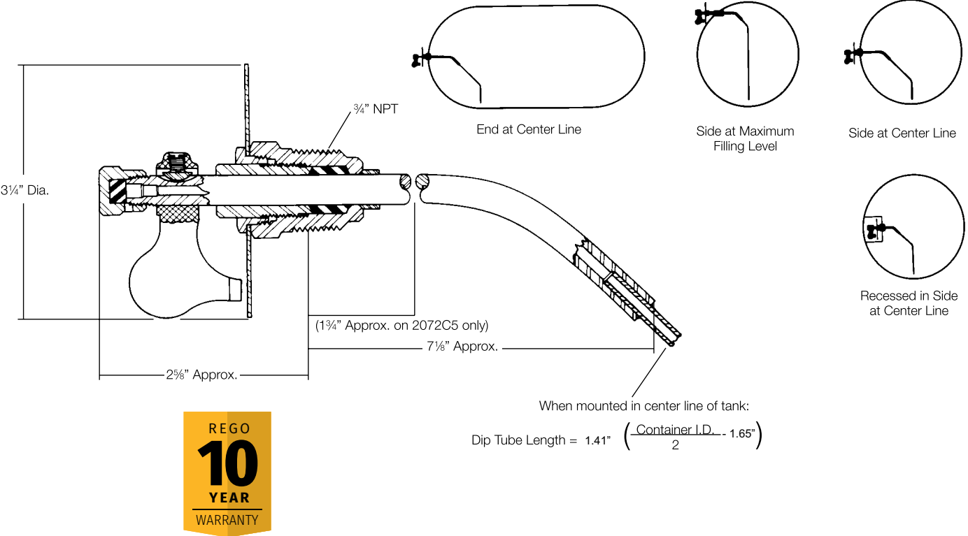
2070 Series Rotogage® Mounting Positions
