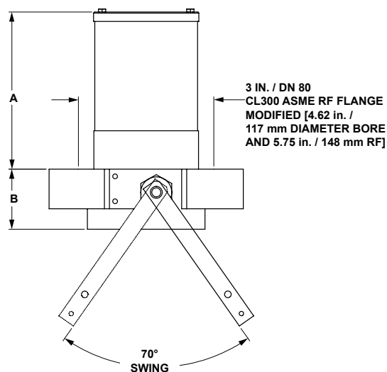
TYPES C484-24 AND C884-24
