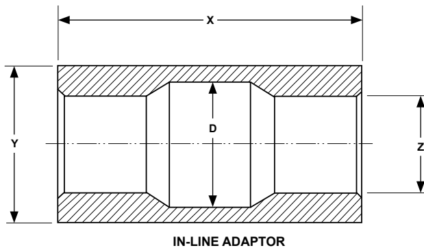
IN-LINE ADAPTOR
