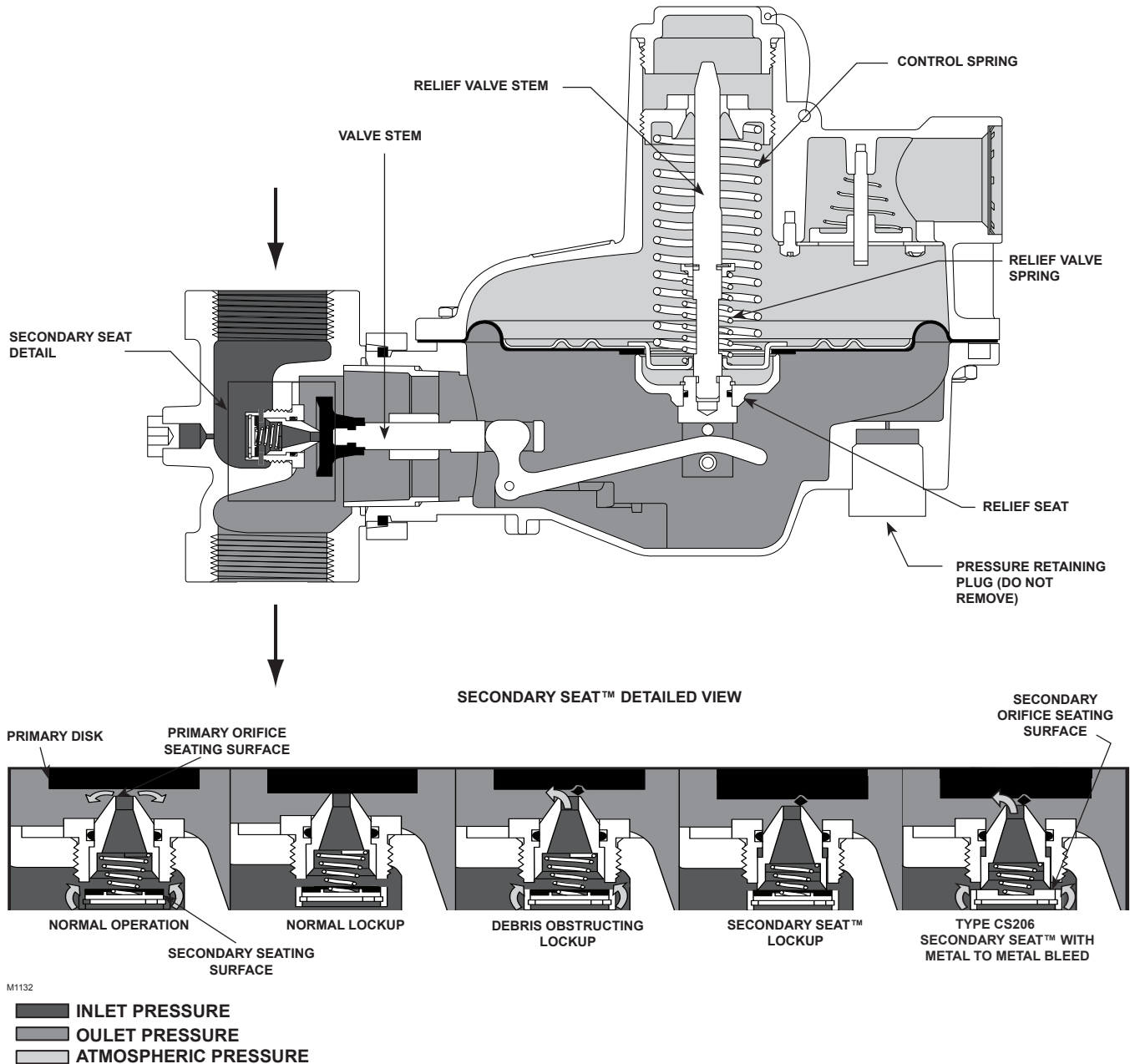
Figure 5. CS200 Series with Secondary Seat Protection
