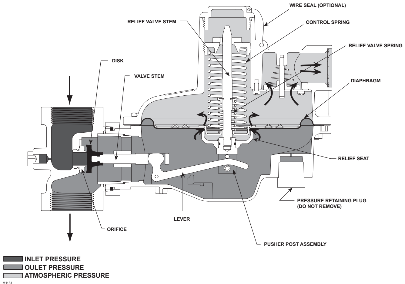
Figure 4. Type CS200IR Pressure Reducing Regulator with Internal Relief
