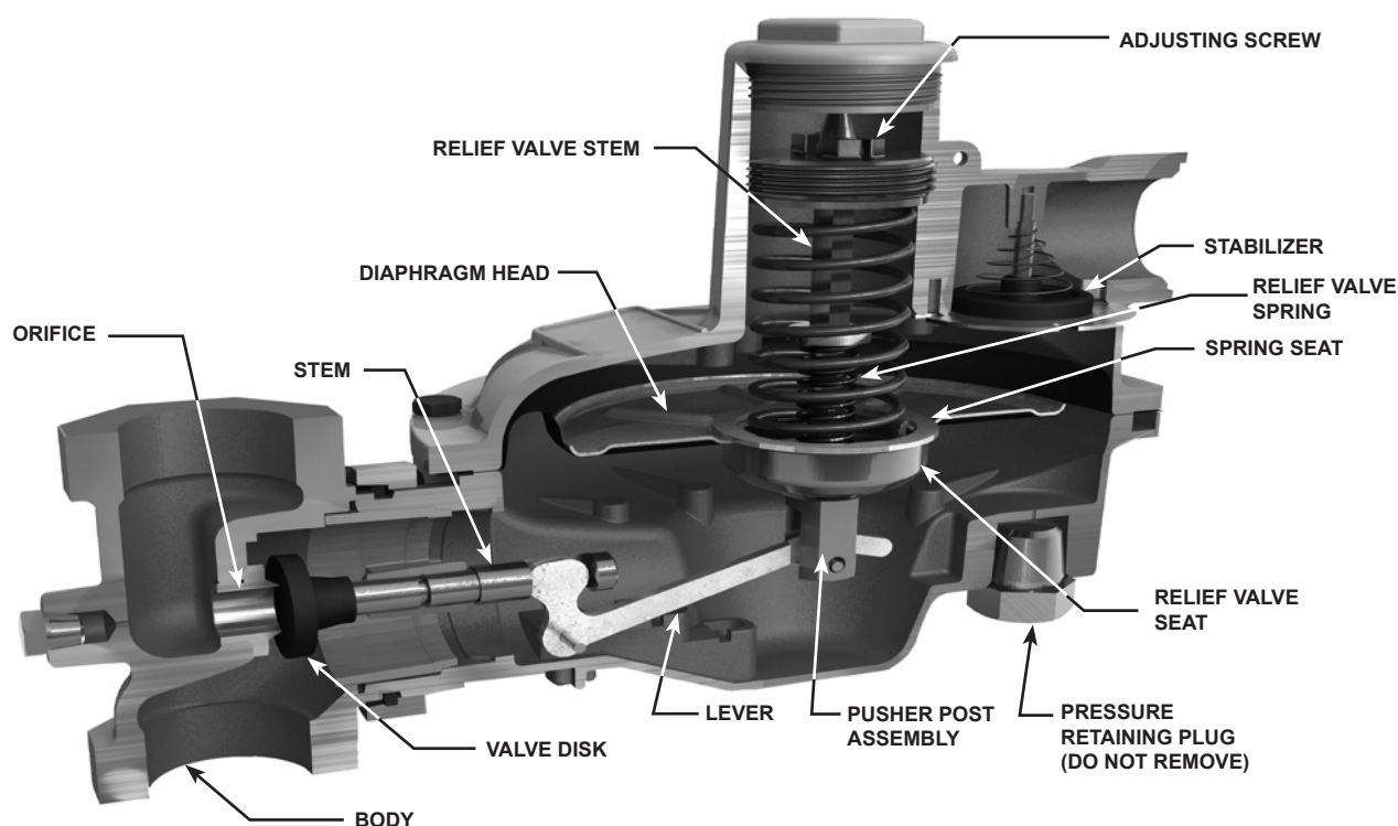
Figure 2. Typical CS200 Pressure Reducing Regulator Cut-Away View
