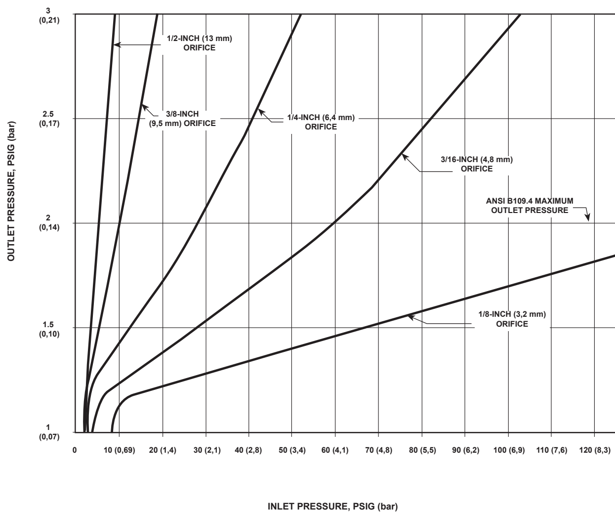
Figure 7. NPS 1 Body Type CS200IR Typical Relief Performance (Linkage Disconnect) at 14-inches w.c. (35 mbar) Set Pressure
