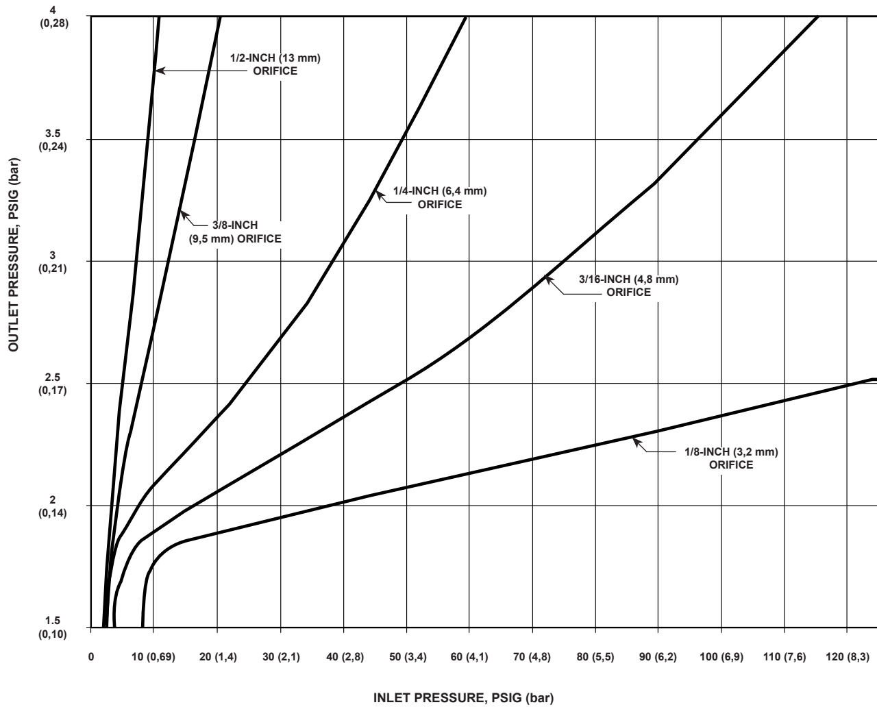
Figure 8. NPS 1 Body Type CS200IR Typical Relief Performance (Linkage Disconnect) at 1 psig (0,07 bar) Set Pressure
