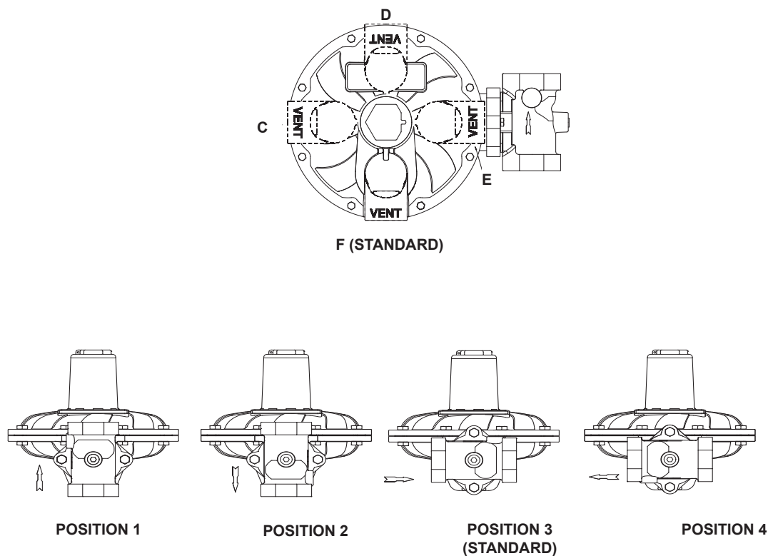
Figure 10. Spring Case Vent and Body Orientation
