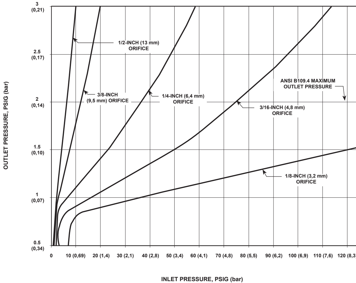
Figure 6. NPS 1 Body Type CS200IR Typical Relief Performance (Linkage Disconnect) at 7-inches w.c. (17 mbar) Set Pressure
