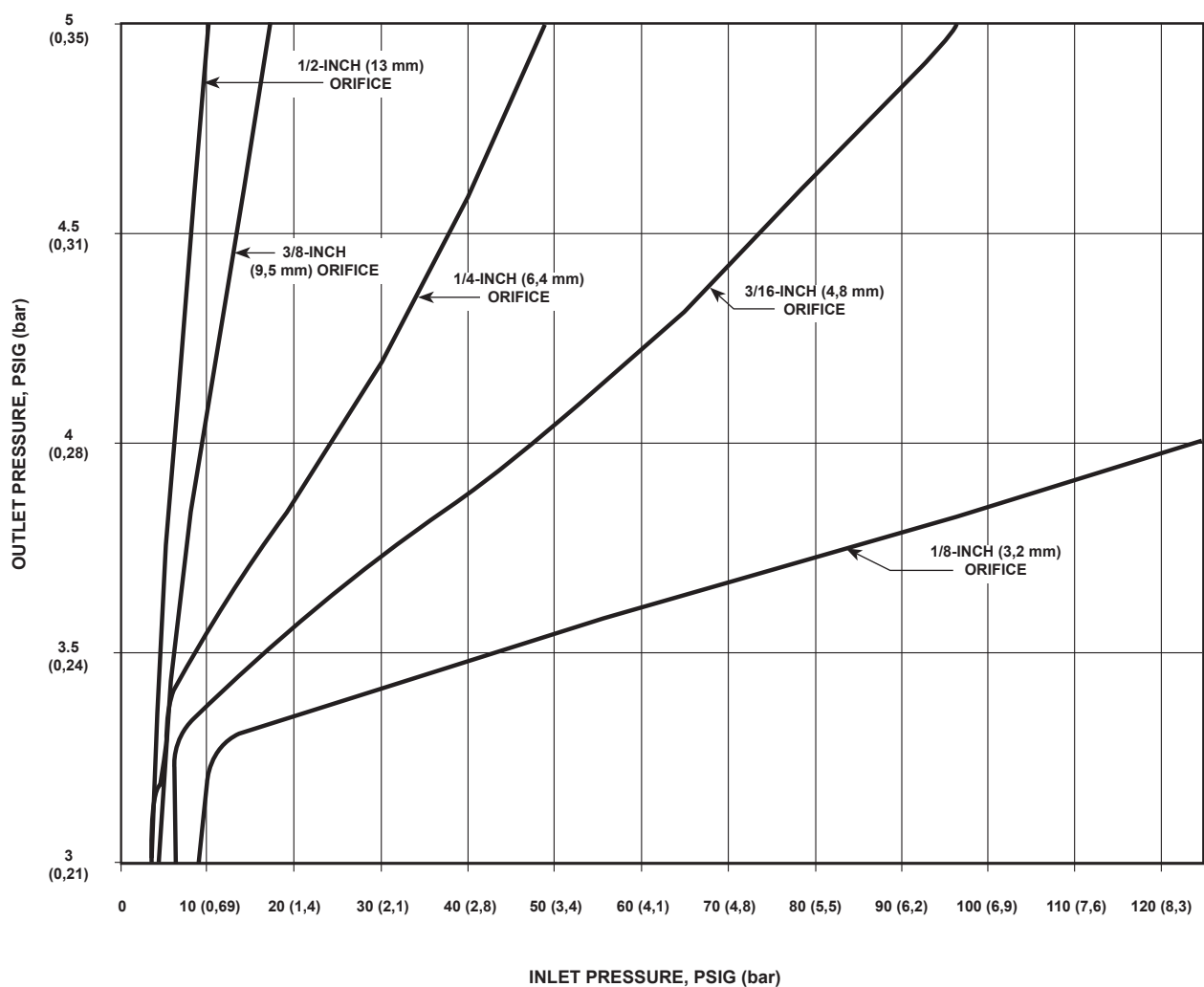
Figure 9. NPS 1 Body Type CS200IR Typical Relief Performance (Linkage Disconnect) at 2 psig (0,14 bar) Set Pressure
