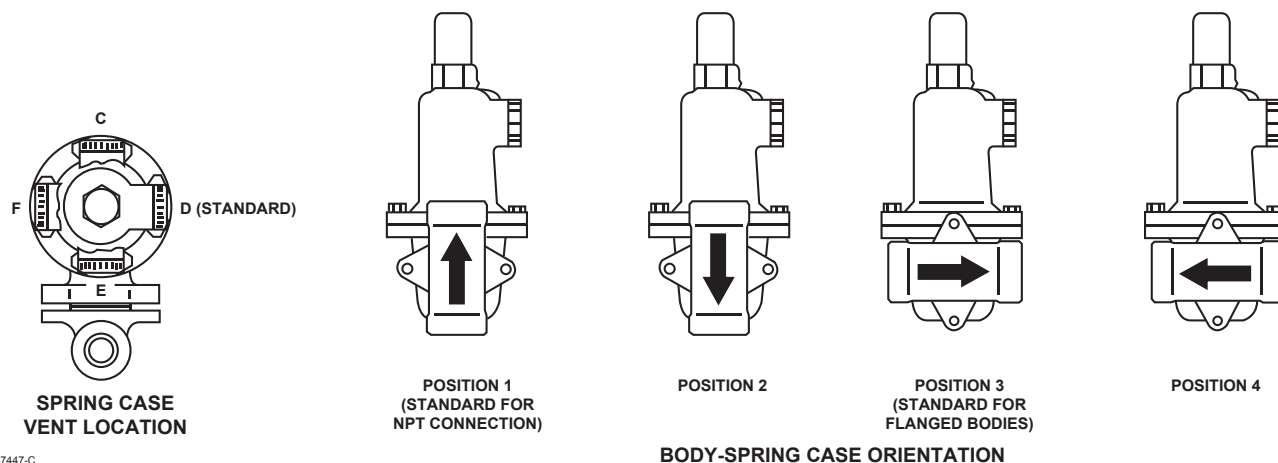
Figure 8. 627 Series Spring Case and Vent Location
