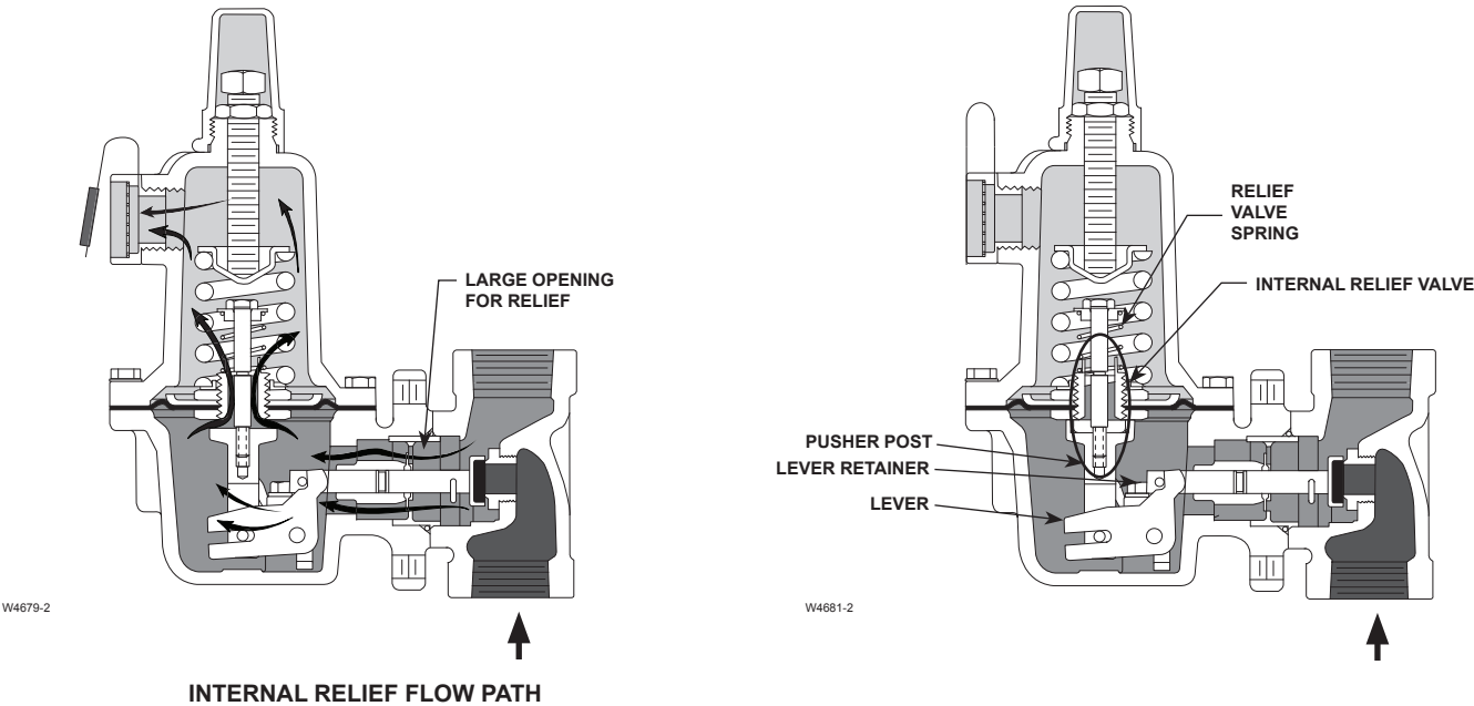
Figure 3. Types 627R and 627LR Operational Schematics
