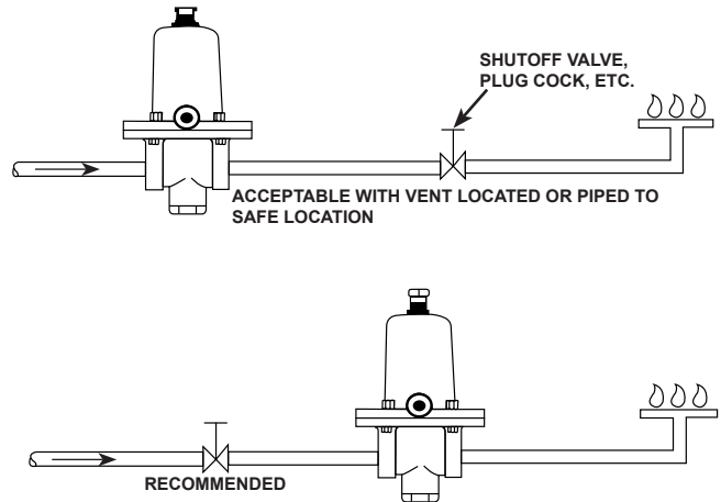
Figure 2. Type 64SR on Liquid Service Requires Care with Downstream Restrictions
